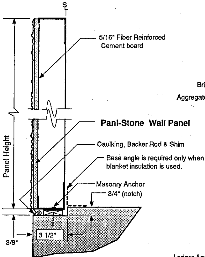
STANDARD BASE DETAIL
