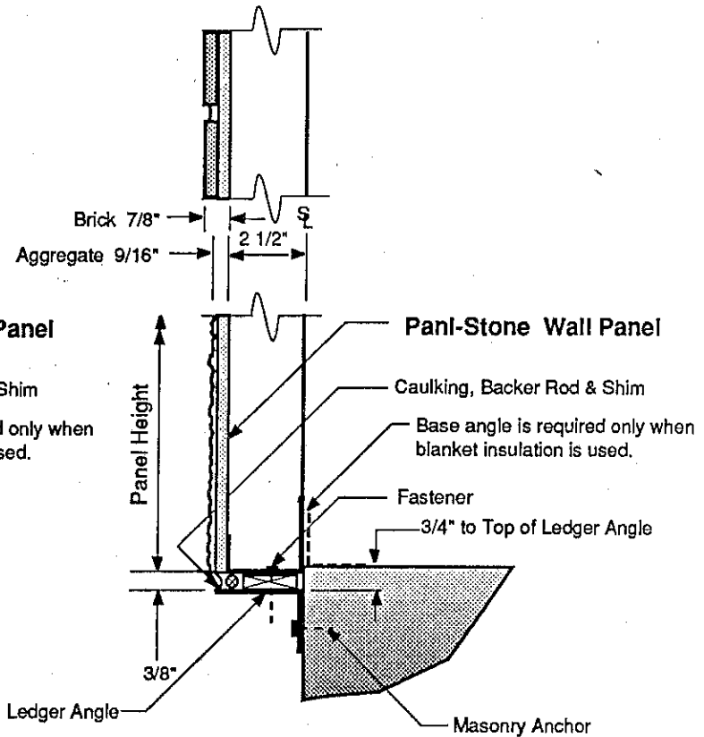
OPTIONAL BASE DETAIL
