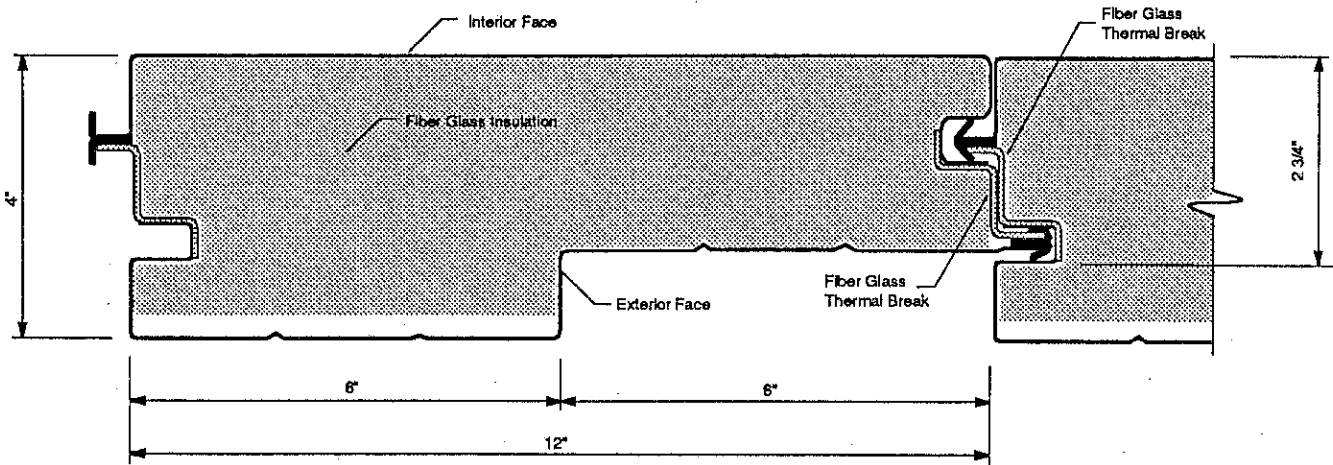
4" THERMAL MONOPANL PANEL CROSS SECTION
