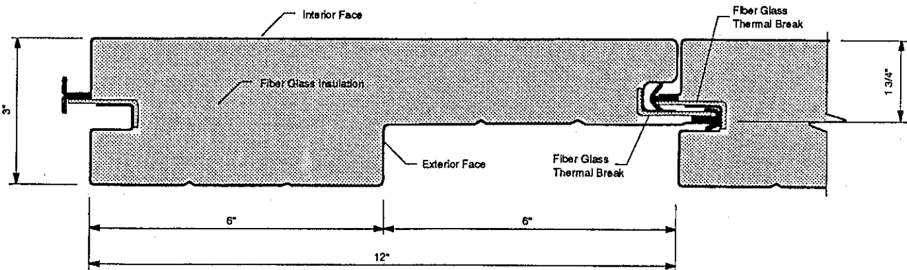
3" THERMAL MONOPANL PANEL CROSS SECTION
