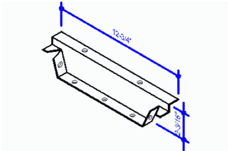
Panel Closure, Butlerrib
