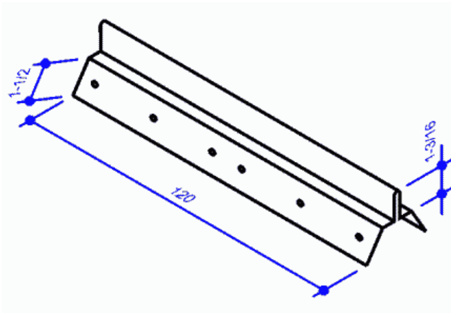
MR-24 Panel Cap PRONTO ® code: 0560361 VISION ® mark: PC10
