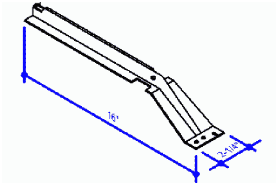
Gutter Support VISION®mark: 0630000
