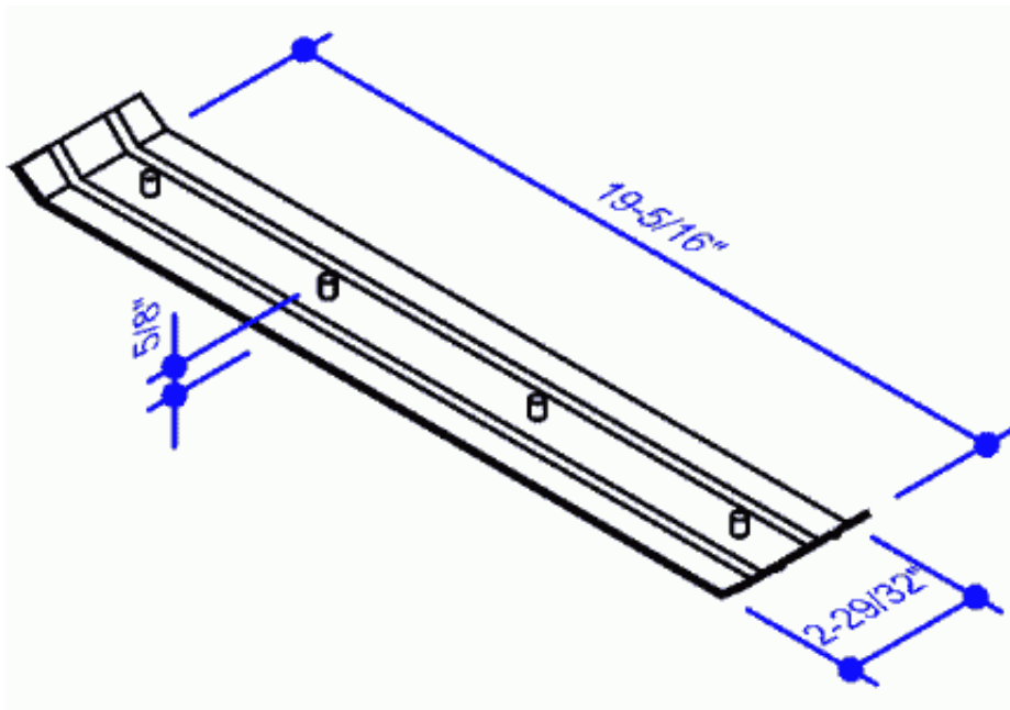
MR-24 Panel Splice Plate Assembly
