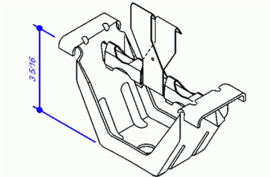
MR-24 Panel Clip Assembly, High
