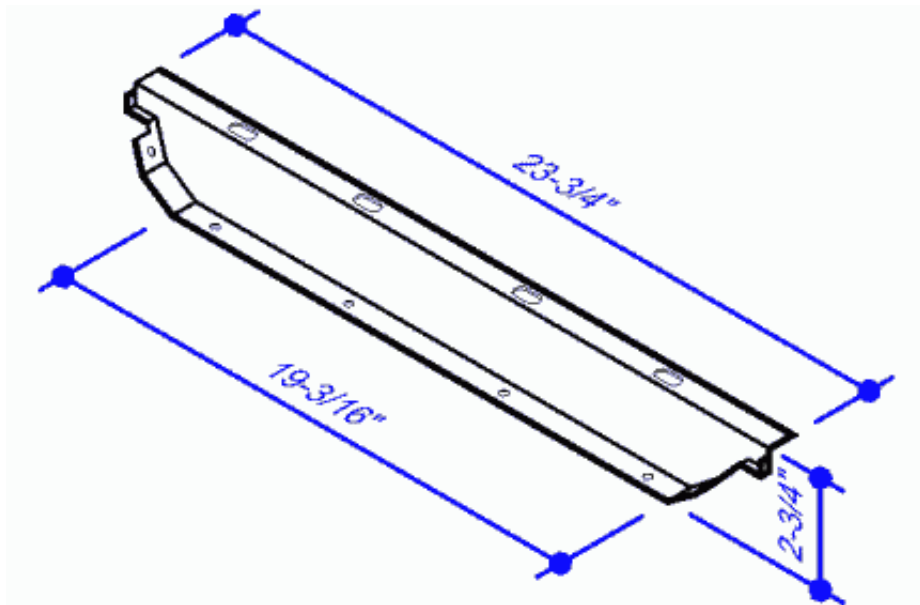
MR-24 Metal Panel Closure
