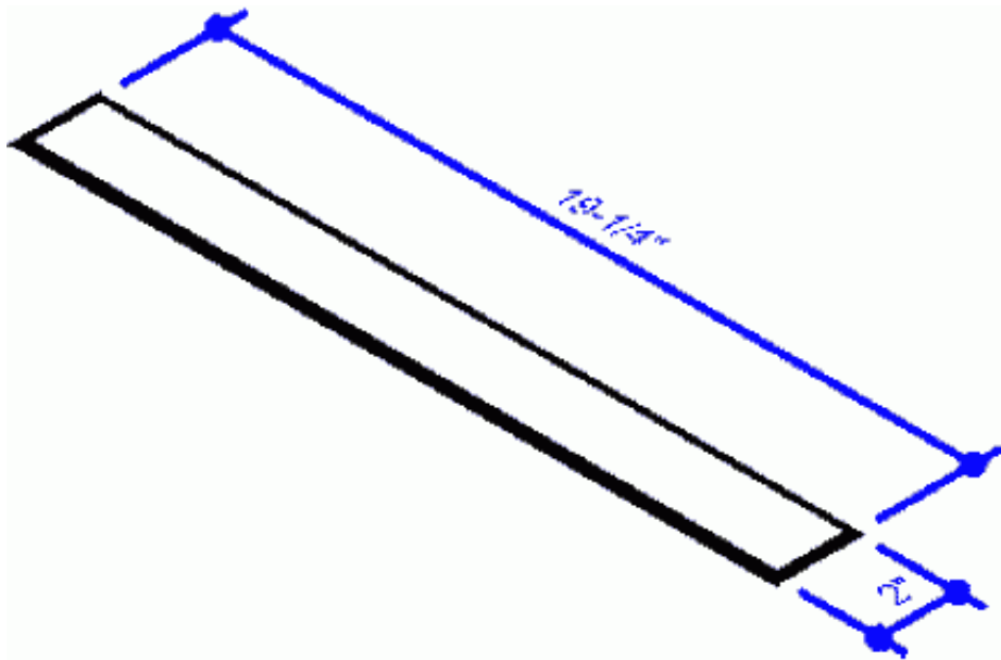
Conductor Strap, 2"x19-1/4" for 4" or 5" Pipe
