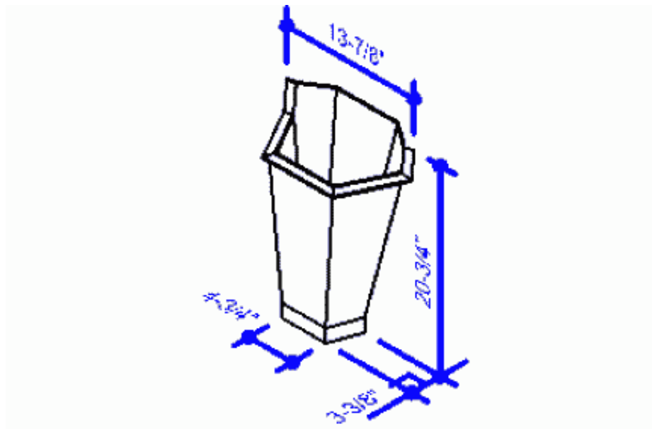
Collector Box for Wide Gutter
