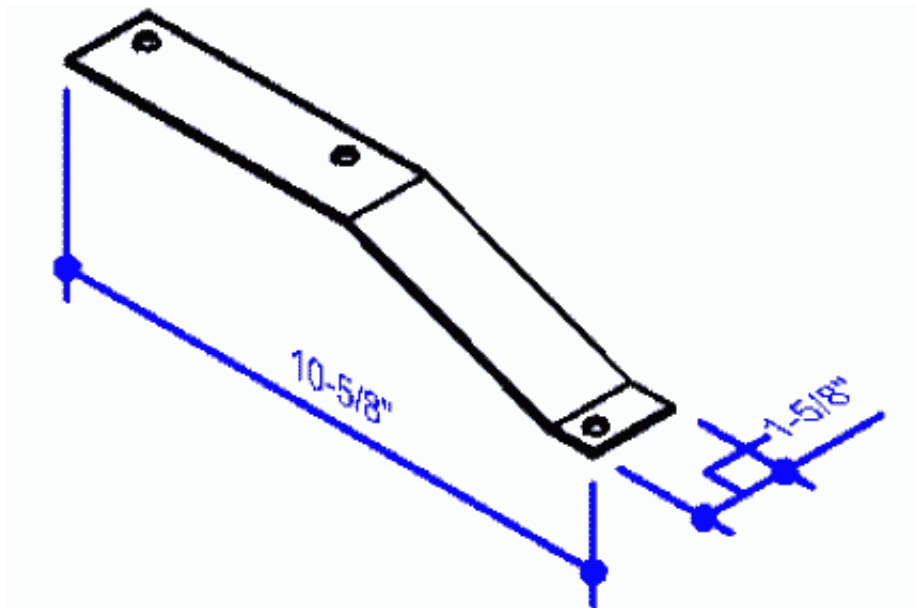
Gutter Hanger 10-29/32" PRONTO ® code: 0630077 VISION ® mark: 0630077
