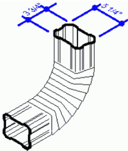
5" Conductor Elbow, 90 Degrees
