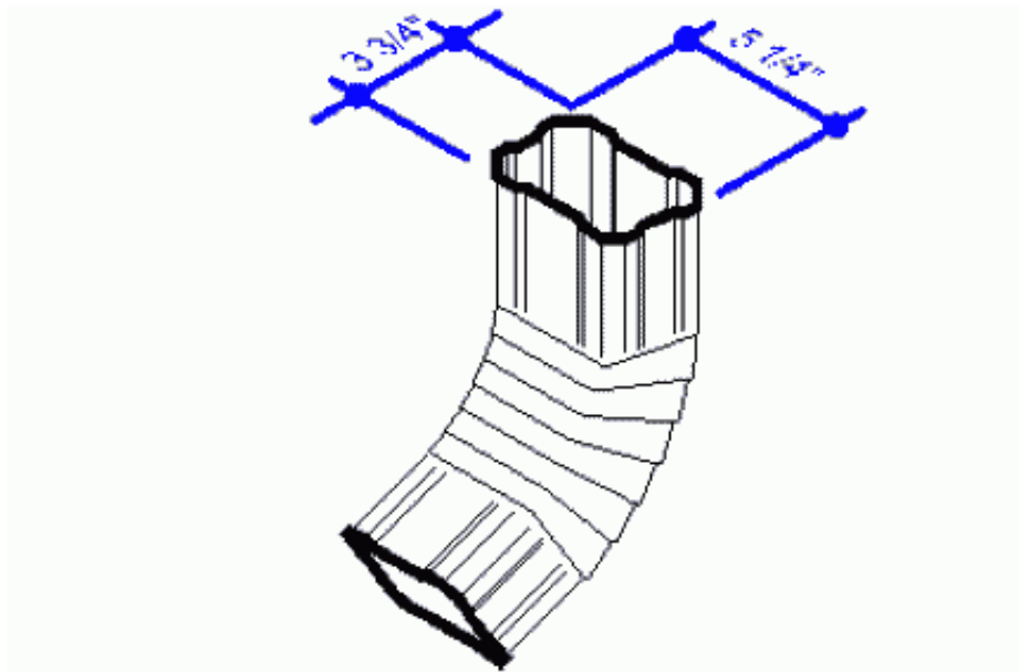
5" Conductor Elbow, 45 Degrees
