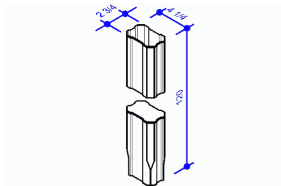
4" Conductor Pipe PRONTO ® code: 0008614 VISION ® mark: CP410
