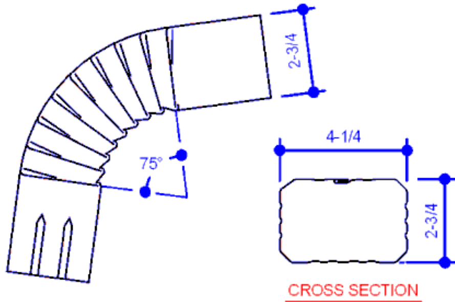
4" Conductor Elbow, 75 Degrees
