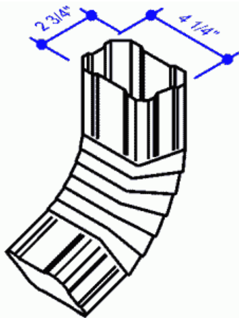
4" Conductor Elbow, 45 Degrees
